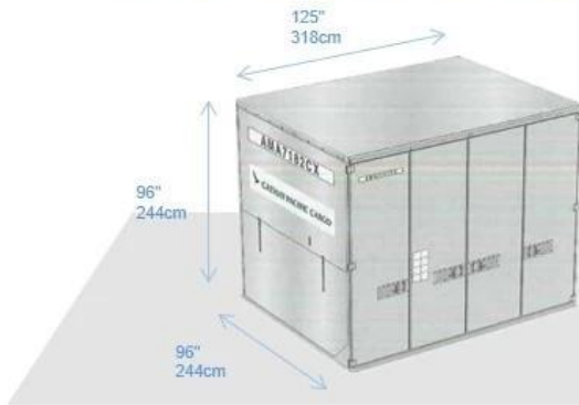
Type: AMA CONTAINER ATA Code: M1 Internal Volume: 621cu. ft 17.58 mc
