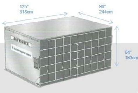
Type: AMA CONTAINER ATA Code: N/A Internal Volume: 406cu. ft 11.5 mc
