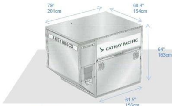
Type: AMA CONTAINER ATA Code: LD3 Internal Volume: 152cu. ft 4.3 mc
